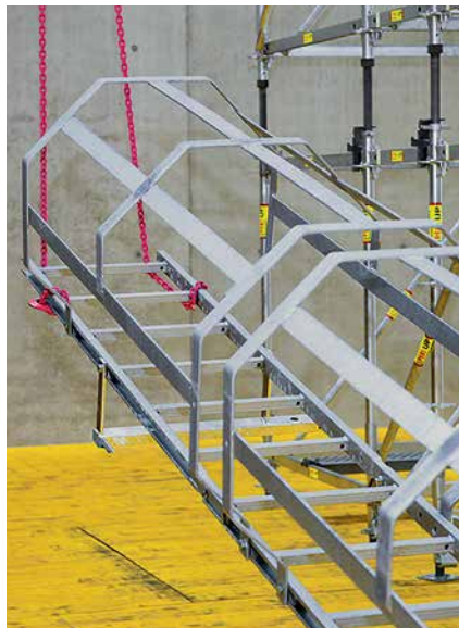
Pre-assembly of the ladder complete with ladder connections and ladder safety cage on the ground.
